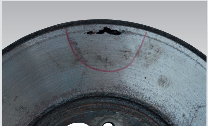
► Blowhole damage
