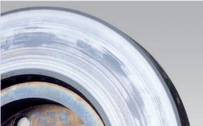
► “Judder marks” through local overheating of brake disc
