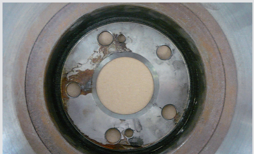
► Cracks in the area of the brake disc chamber
